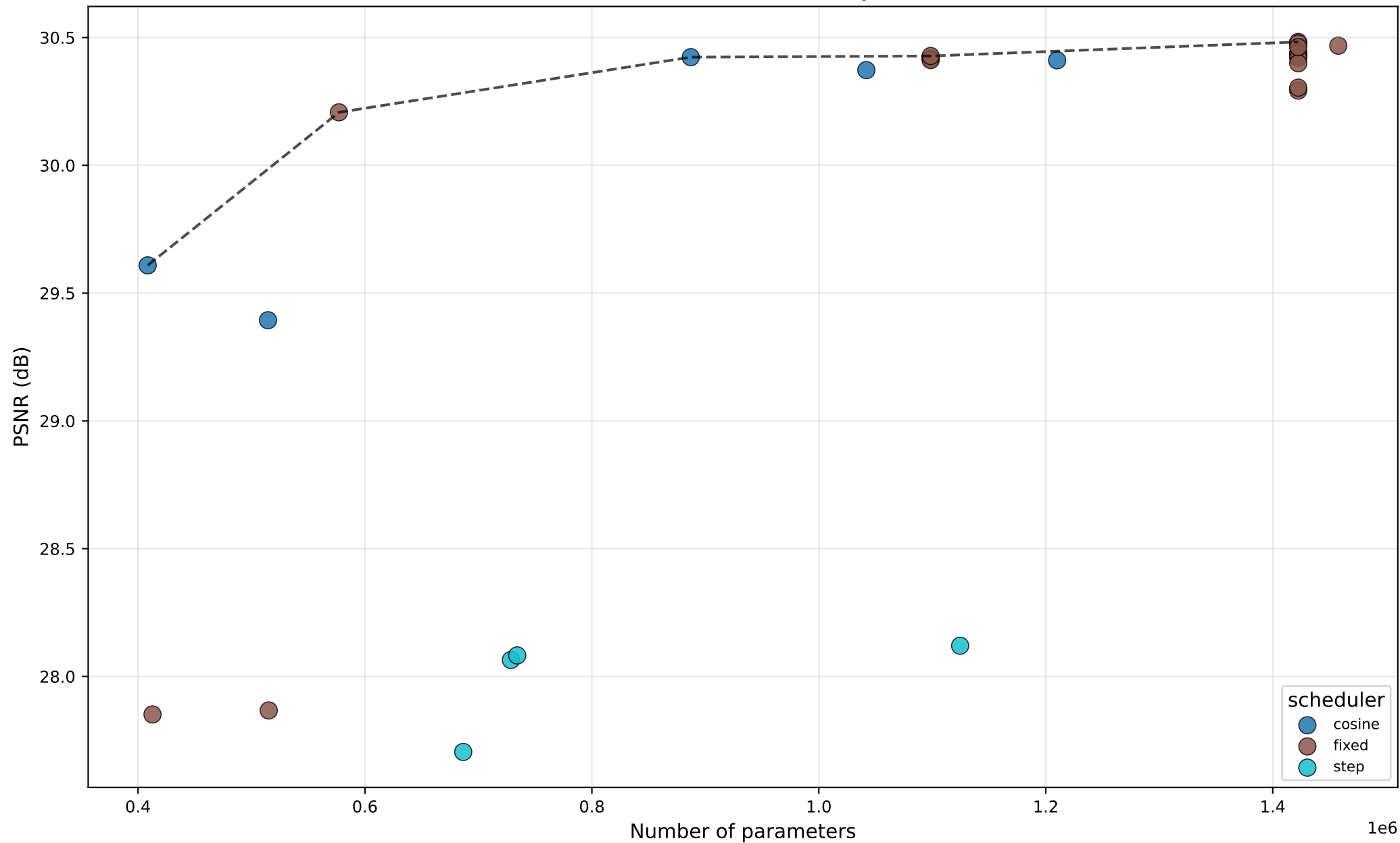
PSNR vs #Params — SwinT — by scheduler
